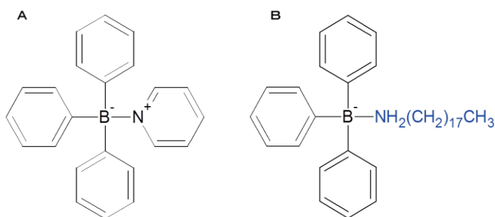
Figure 6. Chemical structures of triphenylborane compounds tested. (A) TPBP (B) TPBOA.
